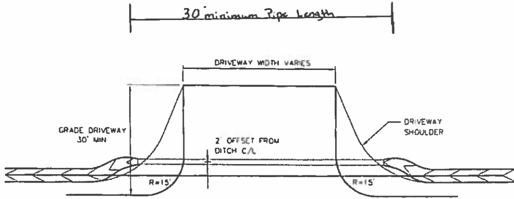
COUNTY ROAD PLAN VIEW NTS
