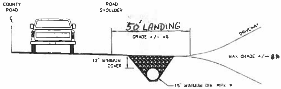
DRIVEWAY PROFILE NTS
